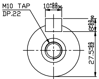
OUTPUT SHAFT
