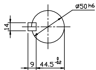
OUTPUT SHAFT
